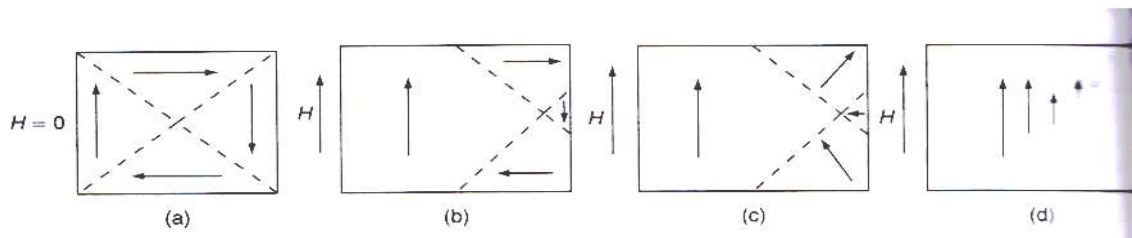
Fig. 6.6 (a) Domain orientation in the absence of the magnetic field (b) Domain enhancement & shrinkage due to weak fields (c) Domain rotation due to strong fields (d) Saturation due to very high fields
