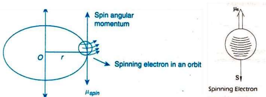
Fig. Spin magnetic moment of electrons
