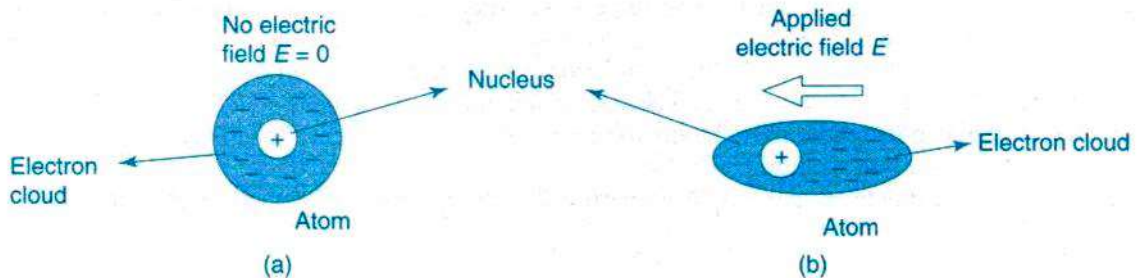
Fig. (a) Un polarized atom in the absence of field (b) Electronic polarization due to distortion of electron cloud by the field E
