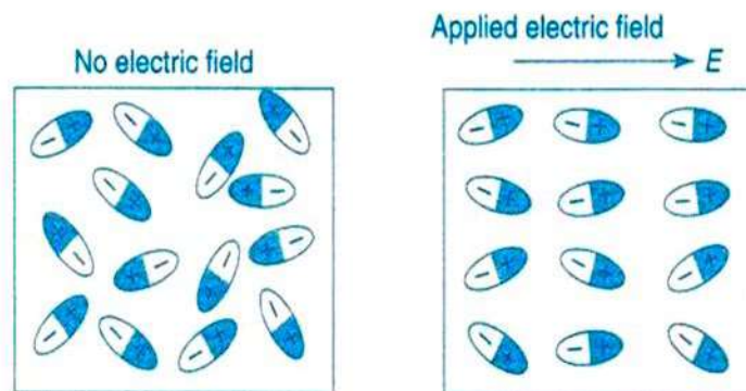
Fig.: Orientalional polarization
