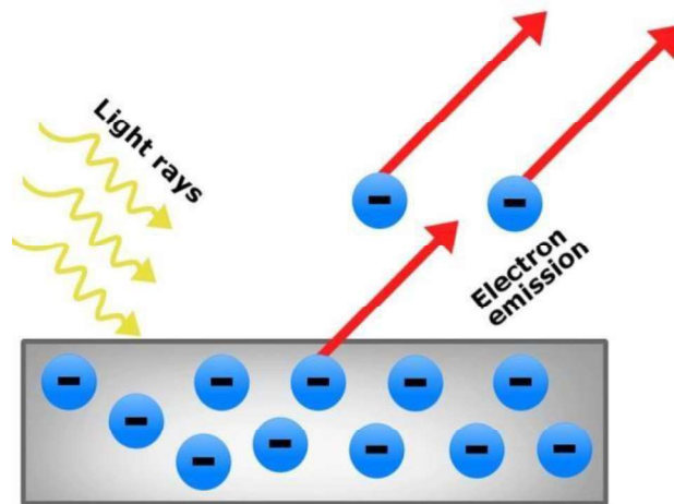
Figure Photoelectric effect
