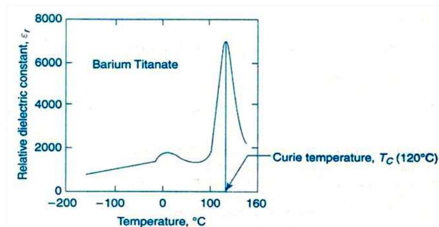
Fig. Variation of dielectric constant with temperature
