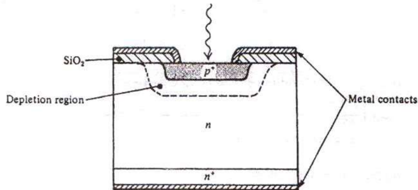
Fig. Typical silicon photo diode structure for photoconductive operation
