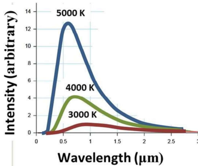
Figure Black body radiation distribution
