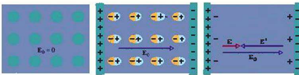
Fig. (a) non polar dielectric in E=0 (b) Non polar dielectric when 'E' is applied (c) Totally polarized non polar dielectric with net field
