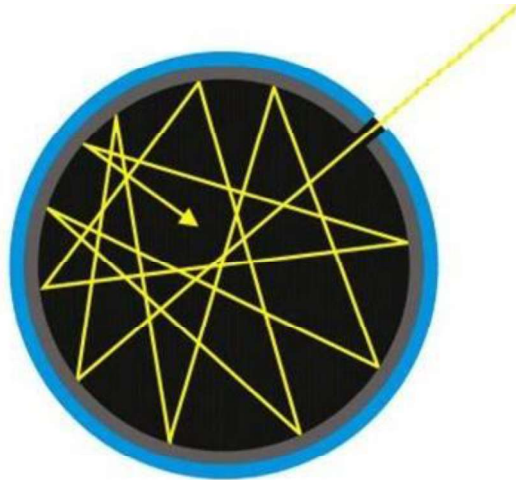
Figure Black body
