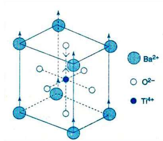
Fig. Structure of \text{BaTiO}_3 above T_c
