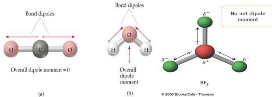
Fig. Non polar molecules with zero dipole moment ( \mu=0 )
