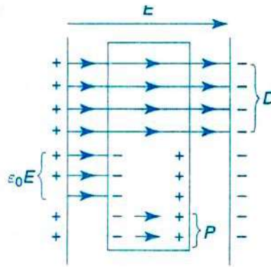
Fig. Electric lines of forces in a polar dielectric
