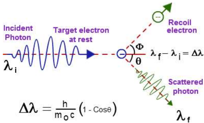
Figure Compton Effect
