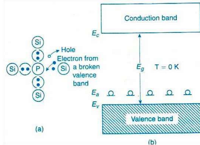
(a) Representation of p- type silicon at T = 0\text{ K} (b) Energy band diagram at T = 0\text{ K}
