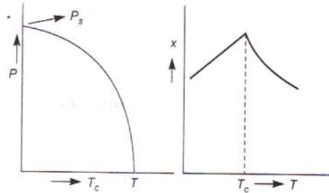
Fig. (a) Spontaneous polarization with respect to temperature (b) Variation of \epsilon_r or \chi with respect to temperature
