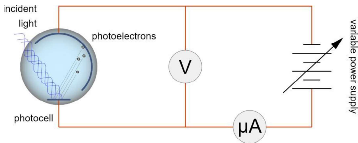
Figure Black diagram of Photo electric effect
