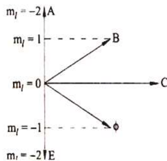
Fig. The three possible orientations of electron
