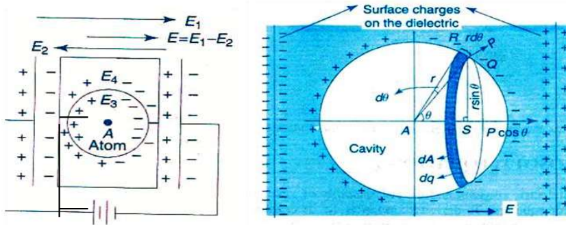
Fig. (a) Polar dielectric in electric field (b) Enlarged view of spherical cavity
