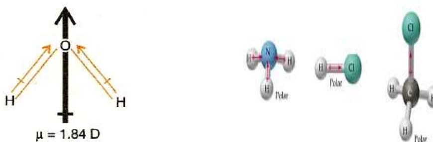
Fig. Polar molecules with net dipole moment ( \mu \neq 0 )
