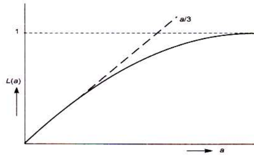
Fig. Langevin curve
