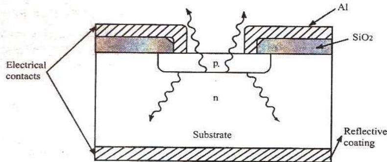
Fig. Construction of typical LED
