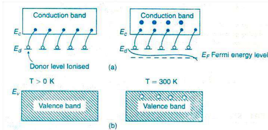
Fig. Variation of Fermi level wrt temperature in n- type semiconductor
