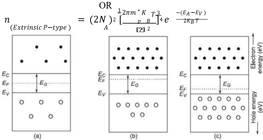
Energy band diagrams of (a) Intrinsic semiconductor (b) N- type & (c) P- type semiconductors
