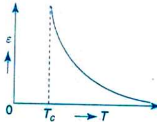
Fig. Variation of dielectric constant with temperature
