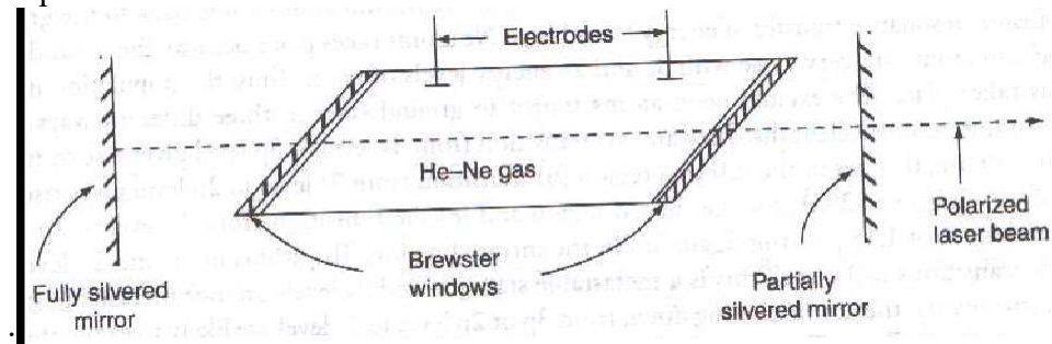
Fig. Helium-Neon gas laser
